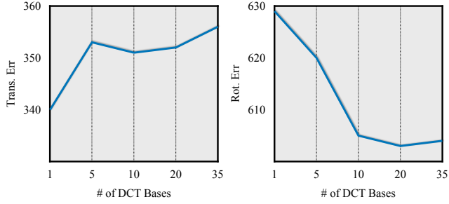
Figure A. Ablation study on the BEHAVE dataset [6]. We evaluate the long-term forecasting where we autoregressively generate 100 frames of future interactions. To balance the performance in predicting rotations and translations, we set the number of DCT bases to 10.
