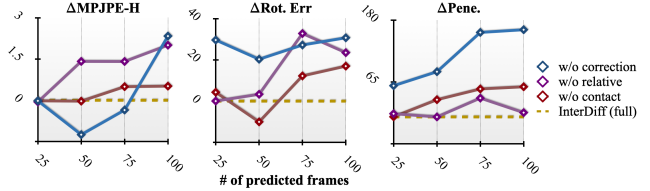
Figure 8. Ablation study on the BEHAVE dataset [6]. We compare our pipeline with various alternatives introduced in Sec. 4.4. We normalize the scores of ‘full model’ to 0. The results show the superiority of ‘full model’ over others in the long horizon.
