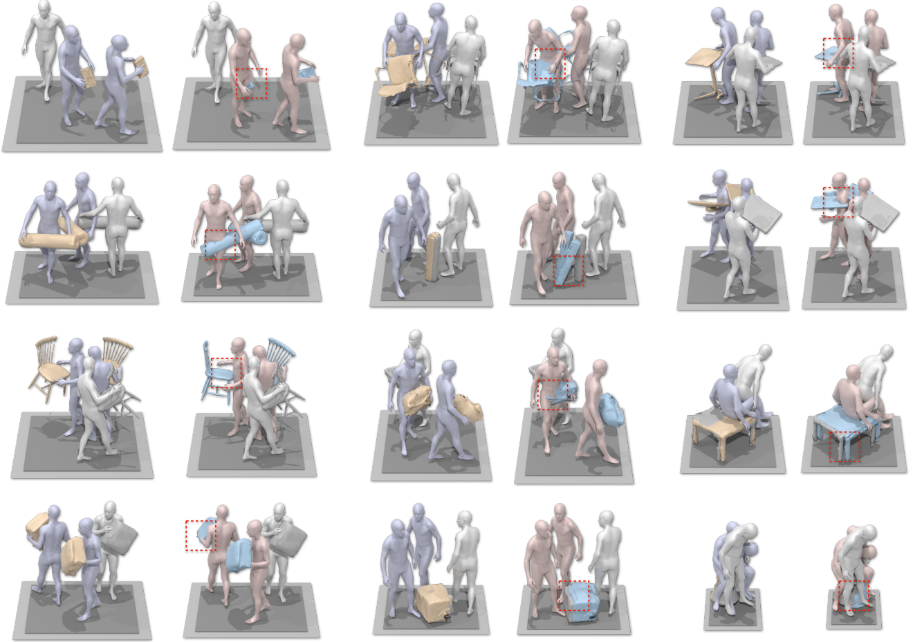
Figure 4. Qualitative comparisons on the BEHAVE dataset [6]. We show starting HOIs in gray and predicted HOIs sampled every 40 frames (30 FPS). The blue and red human meshes denote the results from InterDiff with and without interaction correction, respectively. The injected correction step helps mitigate contact floating and penetration artifacts, and maintain static objects when there is no contact.
