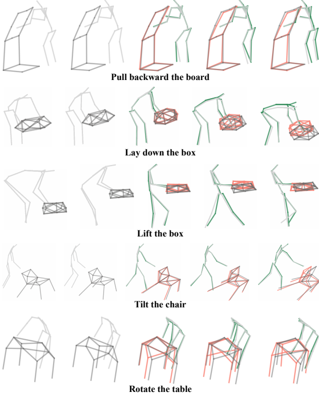
Figure 5. Qualitative results on interactions with unseen objects on the Human-Object Interaction dataset [90]. The predicted skeletons and objects are green and red respectively while GT is gray. We show five frames at 0.4, 0.8, 1.2, 1.6, and 2.0s.
