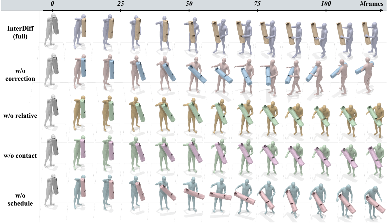
Figure 9. Ablation study on the BEHAVE dataset [6]. We show starting HOIs in gray and predicted HOIs sampled every 10 frames (30 FPS), up to 4 seconds. The ablated variants of our InterDiff produce HOIs containing contact floating and penetration artifacts.
